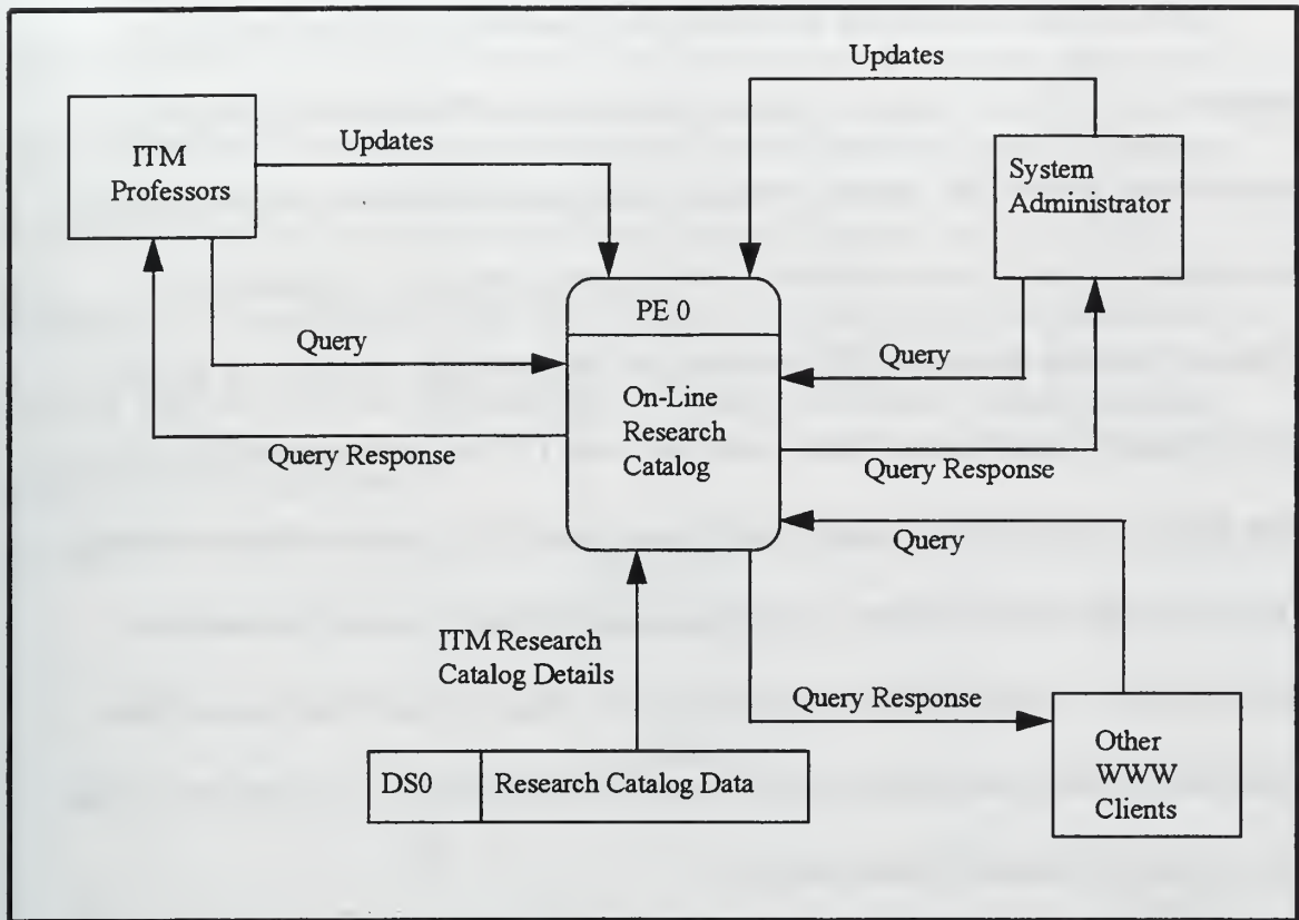
Figure 4. Context Diagram For ITM Research Catalog
